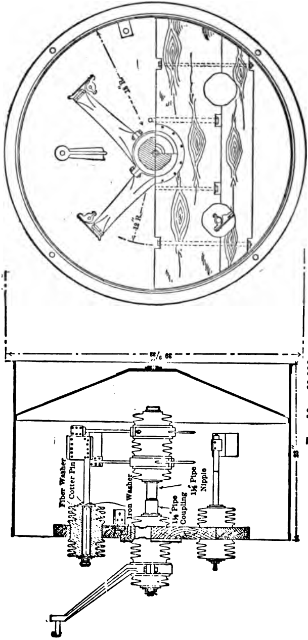
FIG. 10.—60,000-VOLT, FOUR-BREAK, OIL SWITCH.
